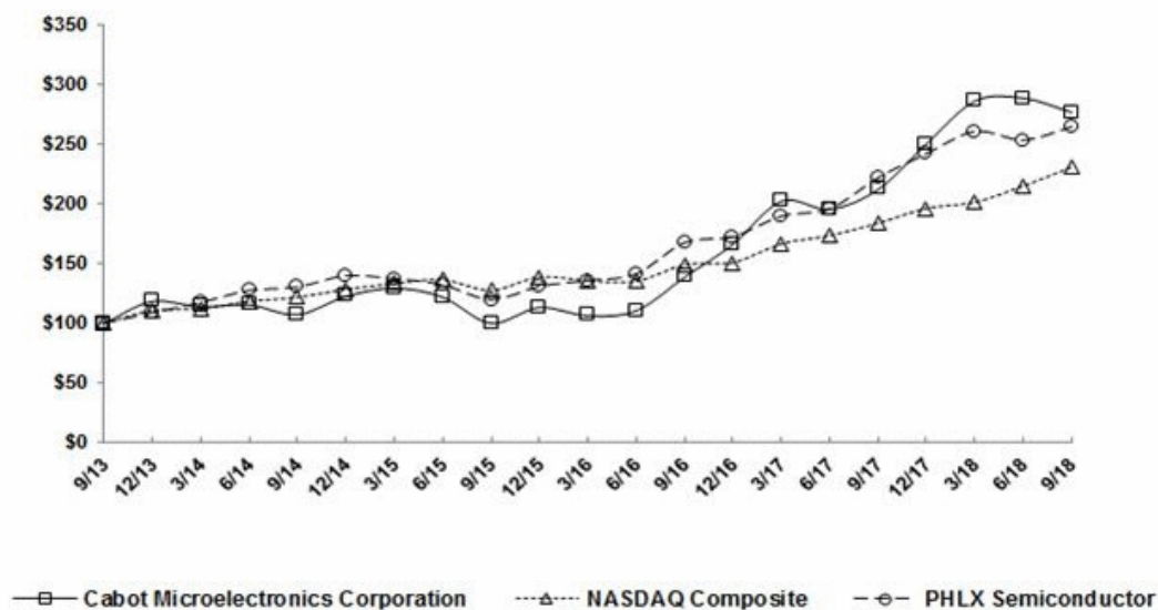
COMPARISON OF 5 YEAR CUMULATIVE TOTAL RETURN* Among Cabot Microelectronics Corporation, the NASDAQ Composite Index and the PHLX Semiconductor Index
